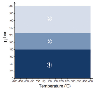
pT diagram for thickness 2.0 mm
