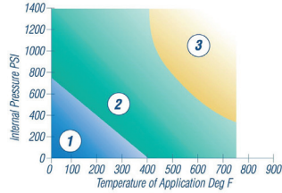
pT diagram for 1/16" thickness
