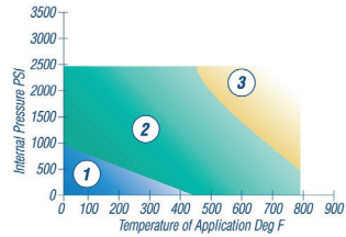
pT diagram for 1/16" thickness
