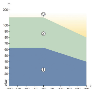
pT diagram for thickness 2.0 mm
