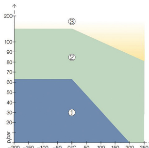
pT diagram for thickness 2.0 mm
