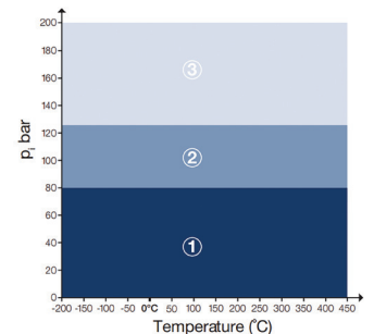
pT diagram for thickness 2.0 mm
